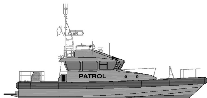
OUTBOARD PROFILE
