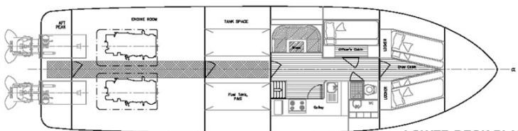
LOWER DECK PLAN
